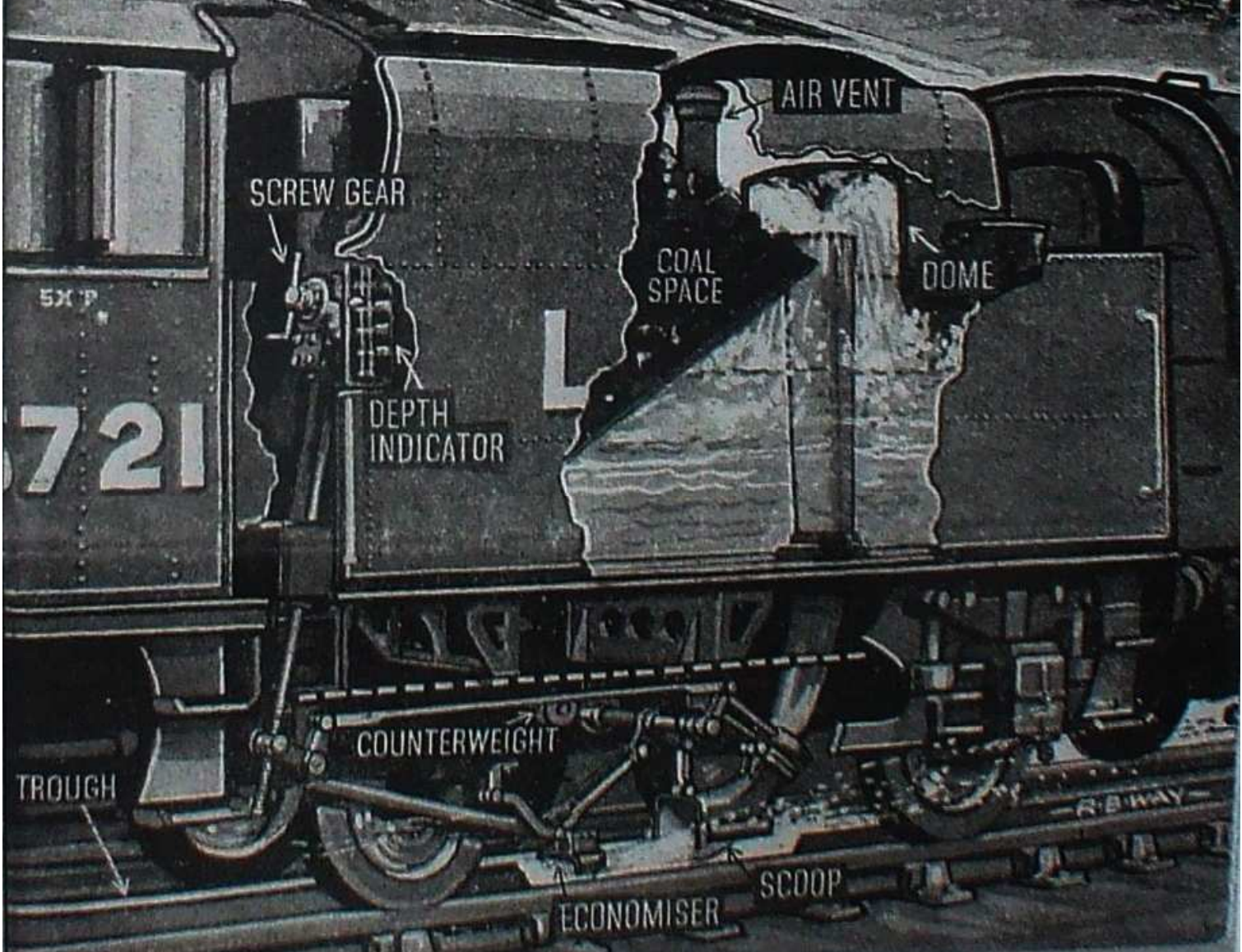
WATER TROUGH CUT TO SHOW SECTION
