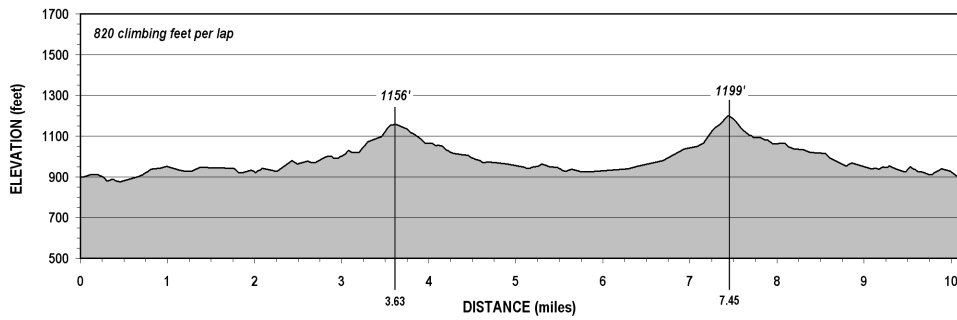
COURSE PROFILE (Vertical exaggeration = 12:1)
