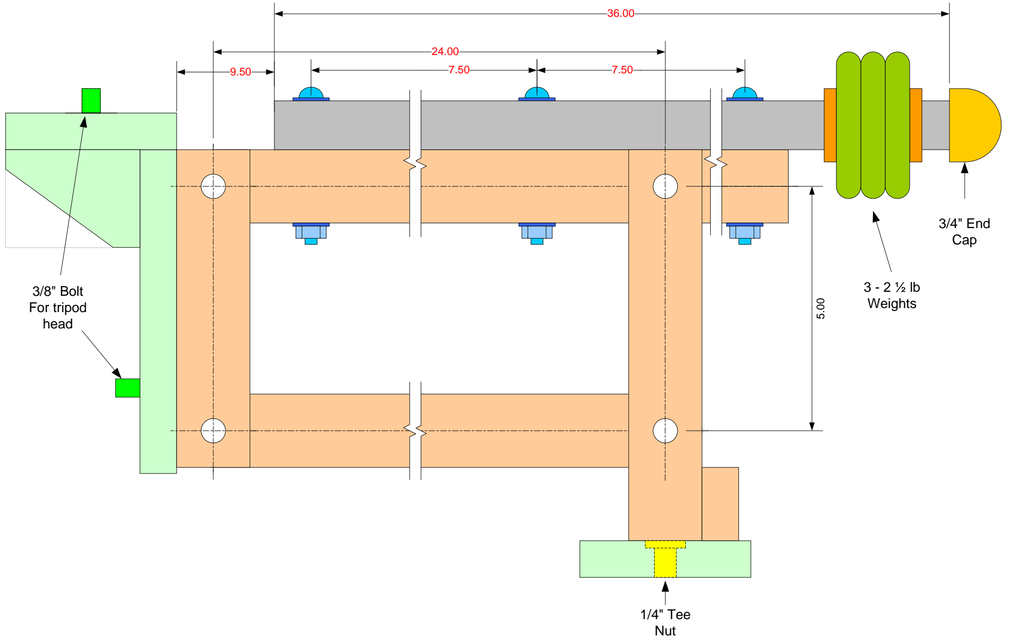
Parallelogram Mount - Complete Assembly
