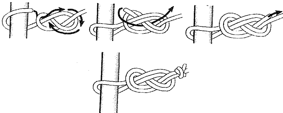
Figure 8 Follow Thru
