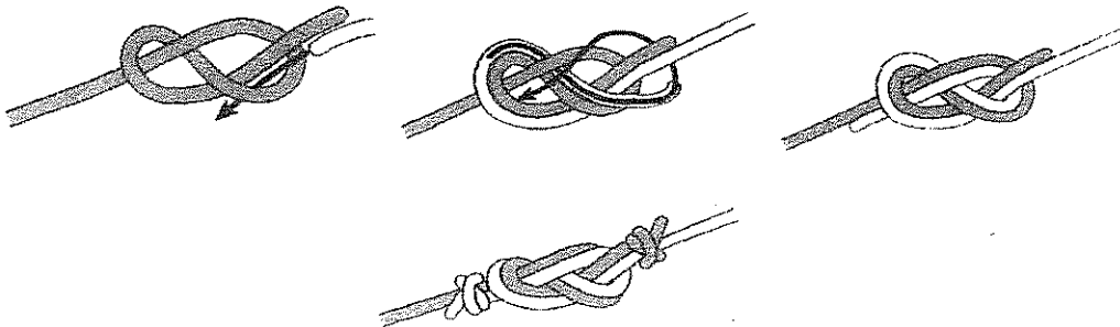
Figure 8 Bend
