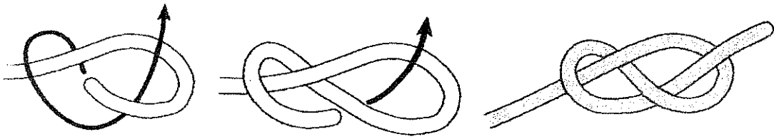
Stopper Knot
